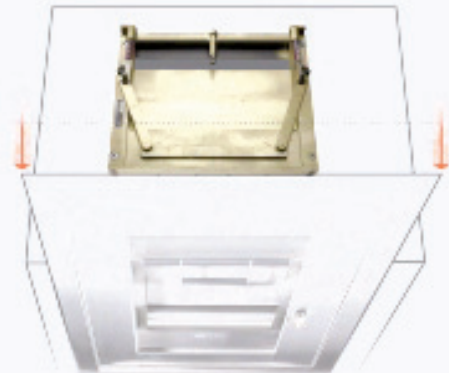
If depository head is removed, closure device snaps shut instantly to deny access to chest and its contents.
